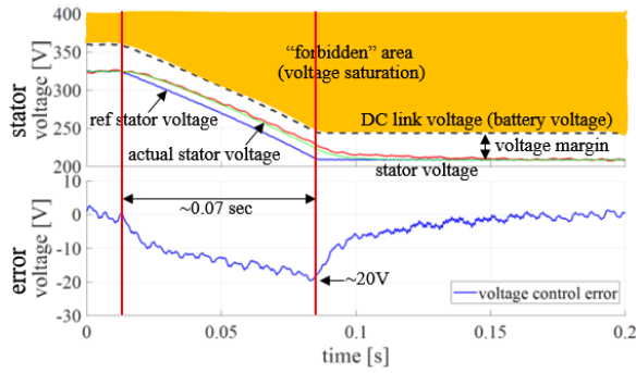
(a) A 0.07 sec change in the DC link voltage causes a 20V error.
