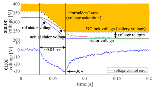
(b) The same voltage change at a faster 0.04 sec rate causes a 30V error.
